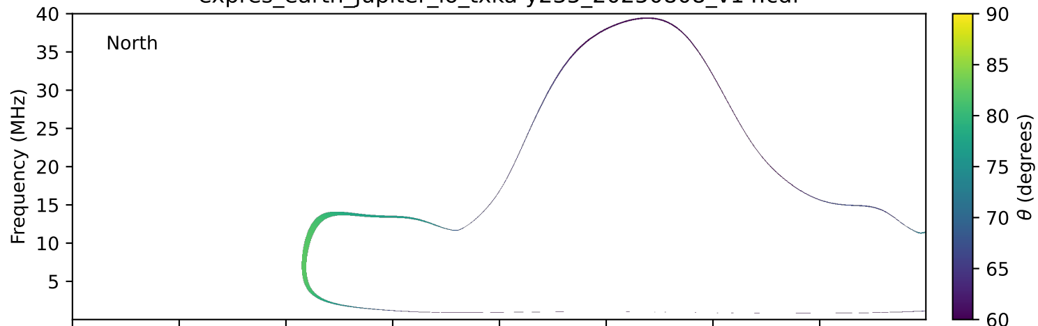
expres_earth_jupiter_io_txka-y235_20250808_v14.cdf
