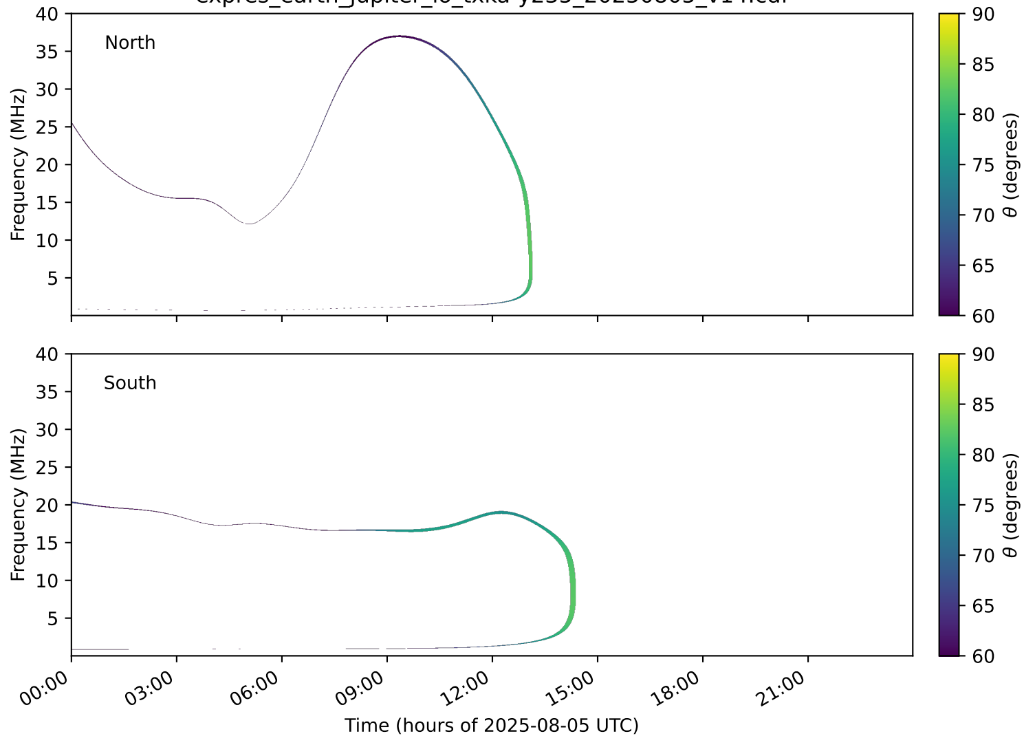
expres_earth_jupiter_io_txka-y235_20250805_v14.cdf
