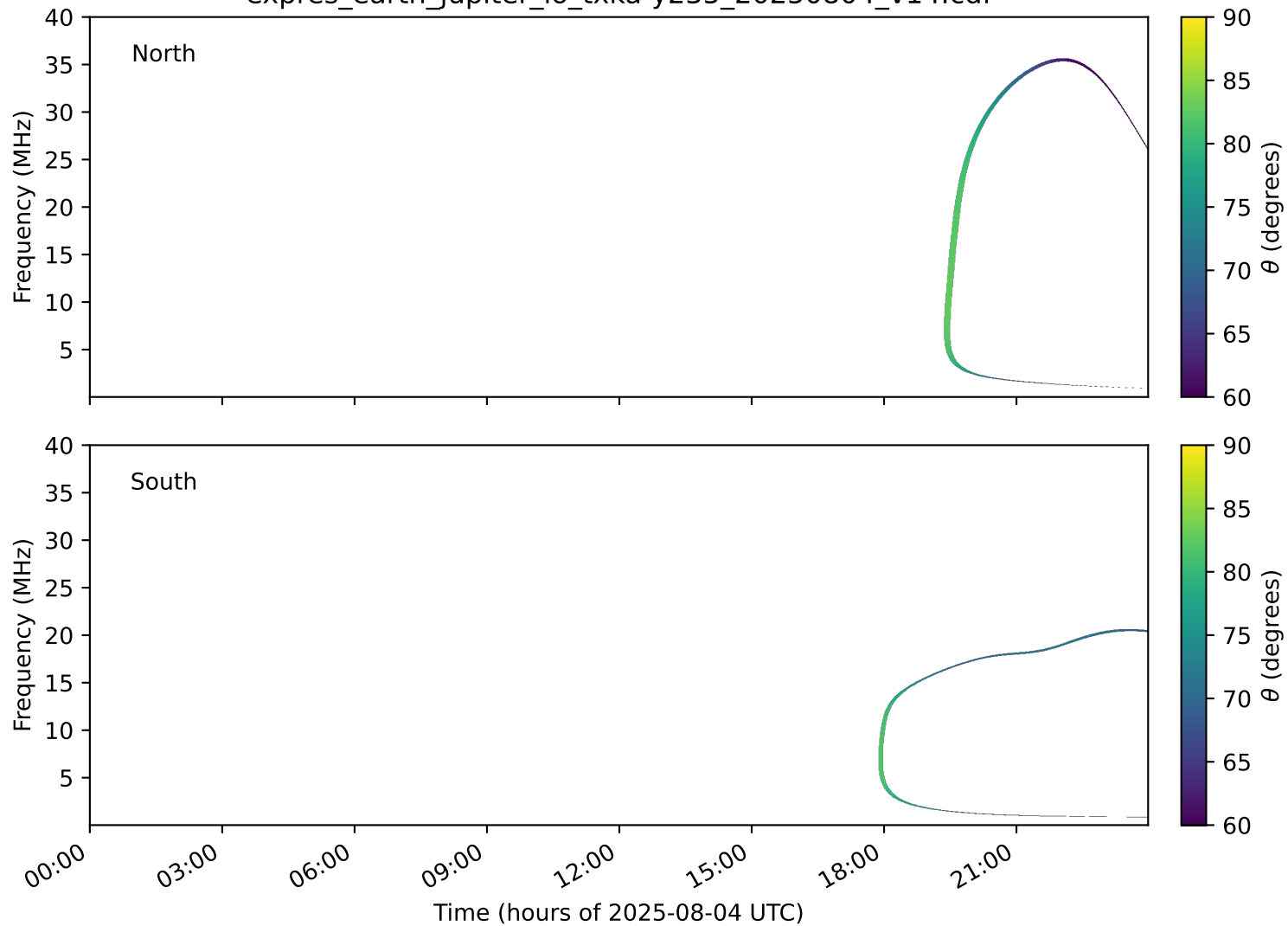
expres_earth_jupiter_io_txka-y235_20250804_v14.cdf
