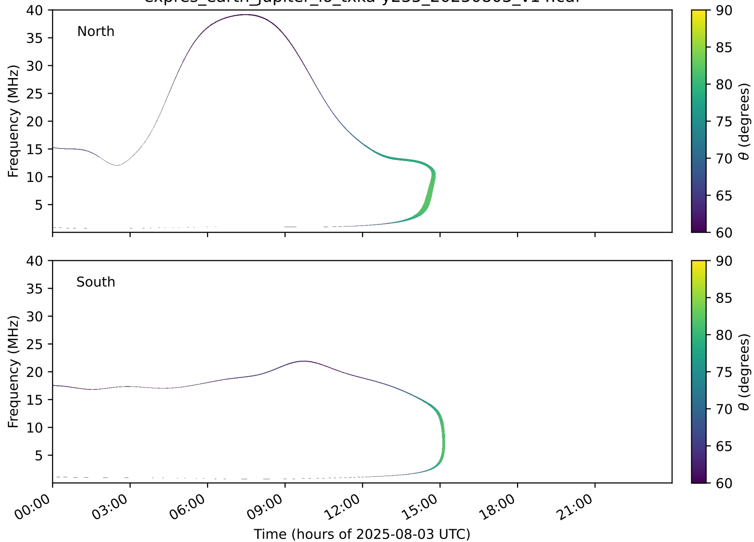
expres_earth_jupiter_io_txka-y235_20250803_v14.cdf
