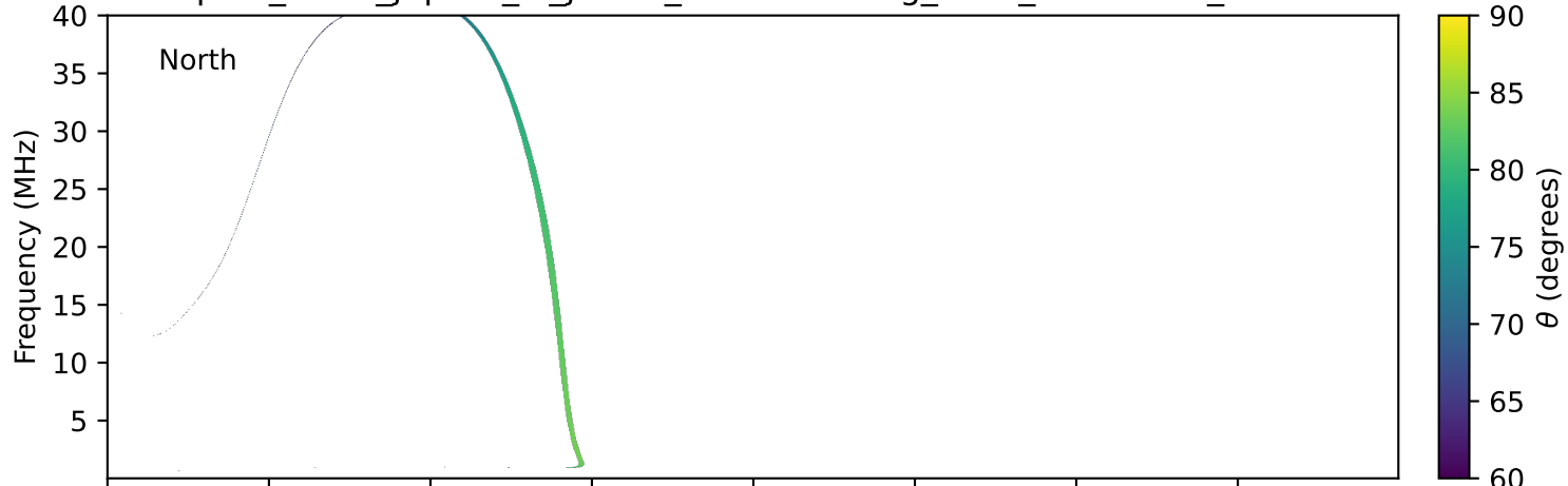
expres_earth_jupiter_io_jrm33_lossc-wid1deg_3kev_20250830_v11.cdf
