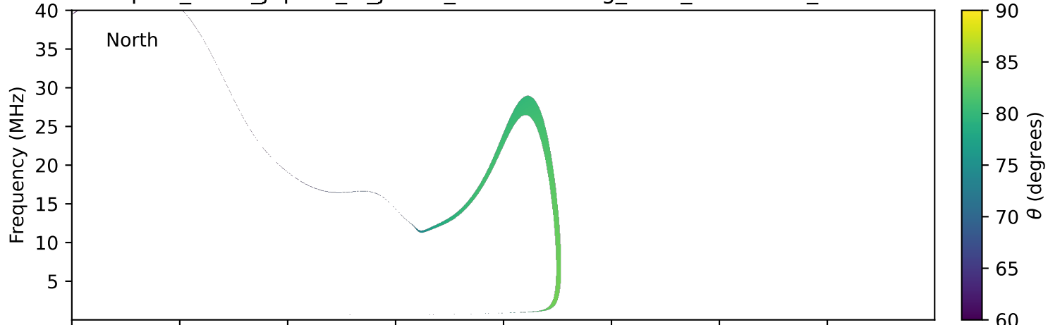
expres_earth_jupiter_io_jrm33_lossc-wid1deg_3kev_20250821_v11.cdf
