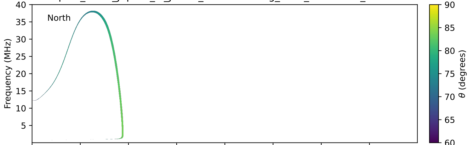
expres_earth_jupiter_io_jrm33_lossc-wid1deg_3kev_20250816_v11.cdf
