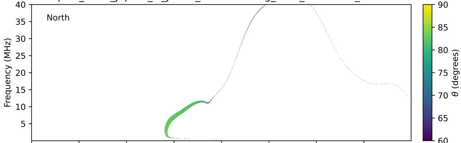
expres_earth_jupiter_io_jrm33_lossc-wid1deg_3kev_20250815_v11.cdf
