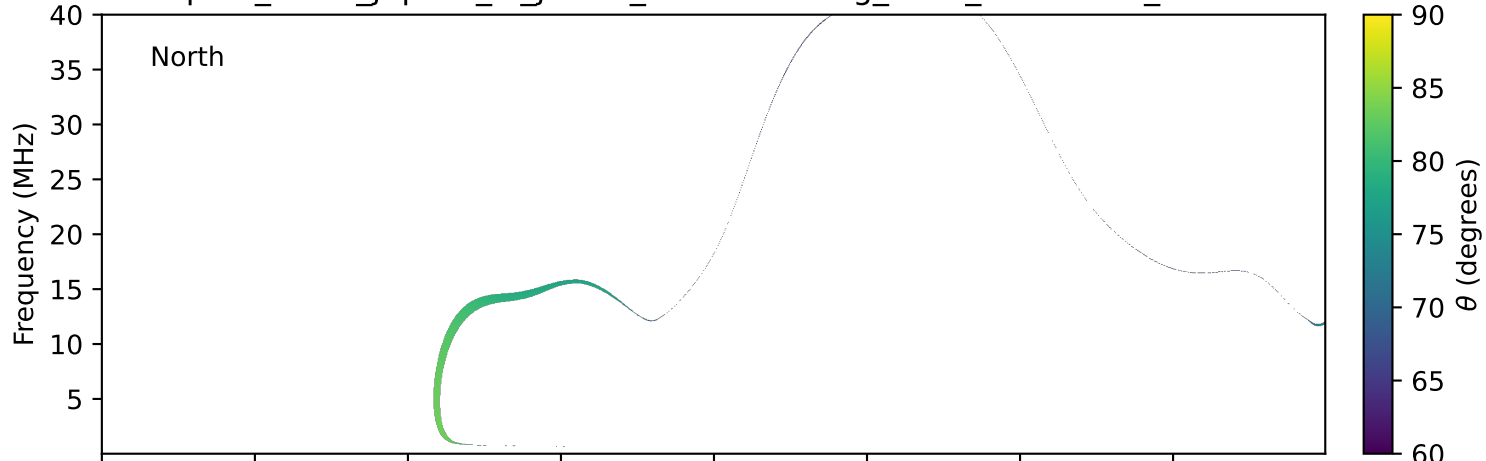
expres_earth_jupiter_io_jrm33_lossc-wid1deg_3kev_20250808_v11.cdf
