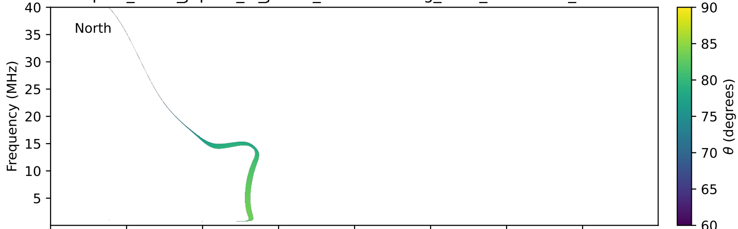
expres_earth_jupiter_io_jrm33_lossc-wid1deg_3kev_20250807_v11.cdf
