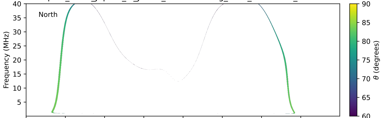
expres_earth_jupiter_io_jrm33_lossc-wid1deg_3kev_20250801_v11.cdf
