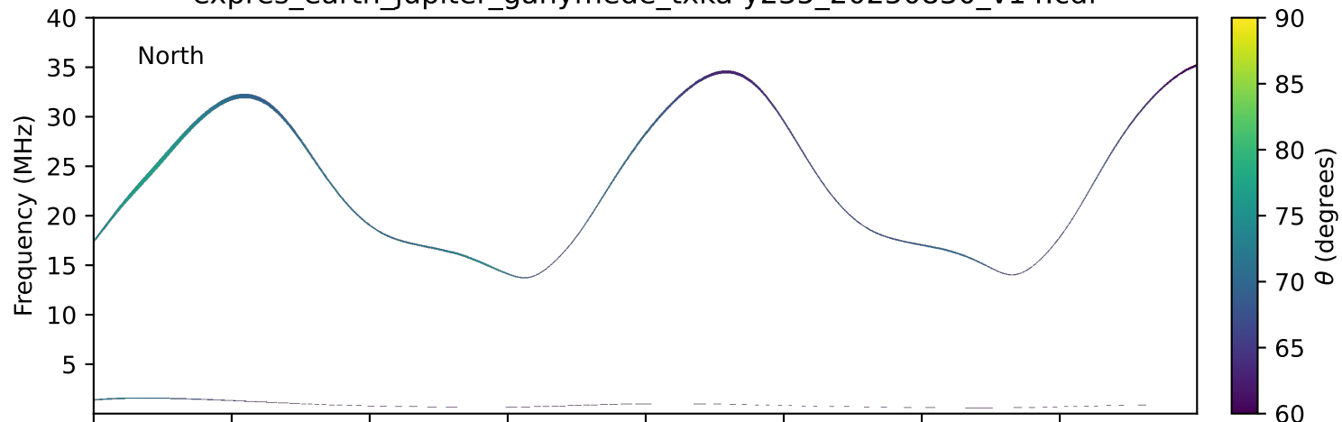
expres_earth_jupiter_ganymede_txka-y235_20250830_v14.cdf
