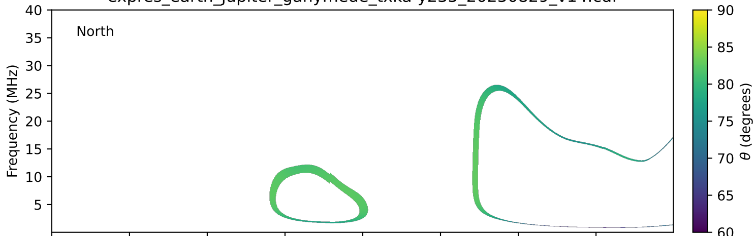
expres_earth_jupiter_ganymede_txka-y235_20250829_v14.cdf
