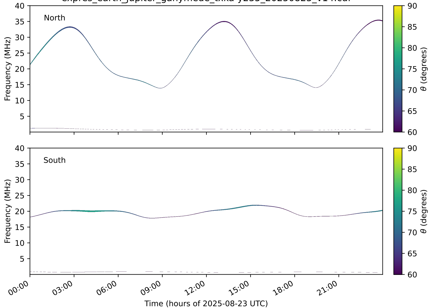
expres_earth_jupiter_ganymede_txka-y235_20250823_v14.cdf
