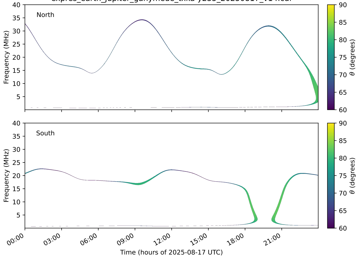
expres_earth_jupiter_ganymede_txka-y235_20250817_v14.cdf
