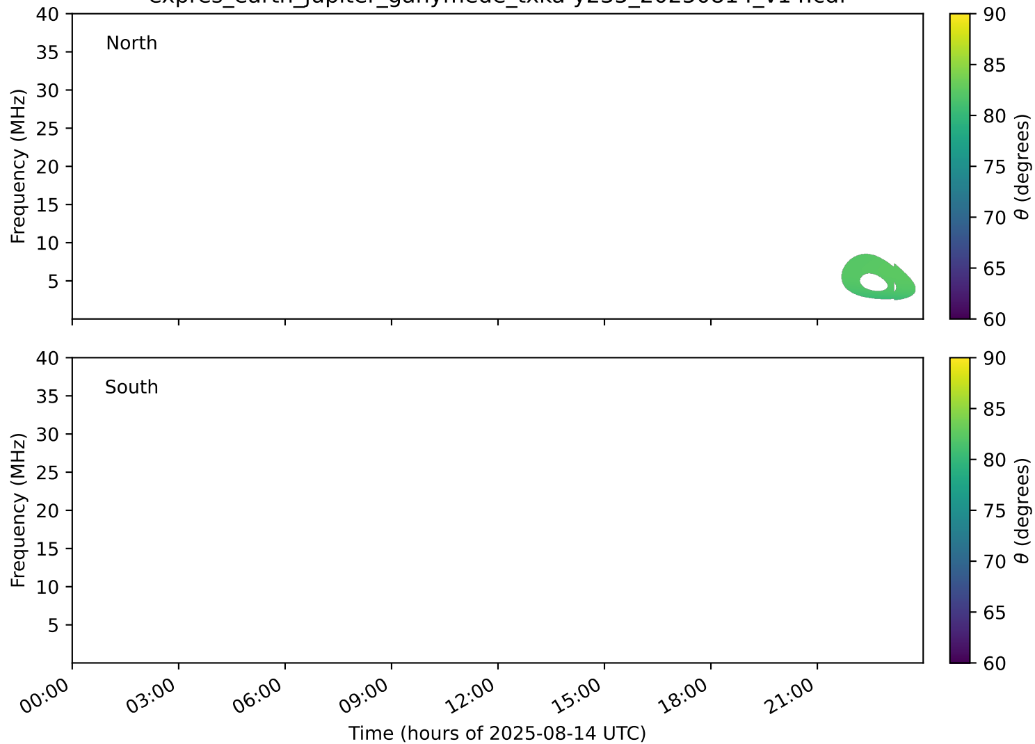
expres_earth_jupiter_ganymede_txka-y235_20250814_v14.cdf
