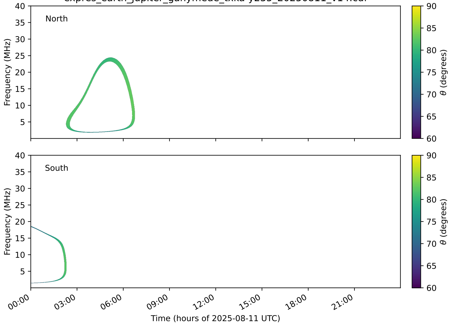
expres_earth_jupiter_ganymede_txka-y235_20250811_v14.cdf
