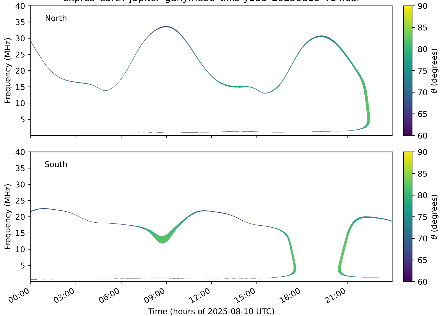
expres_earth_jupiter_ganymede_txka-y235_20250810_v14.cdf
