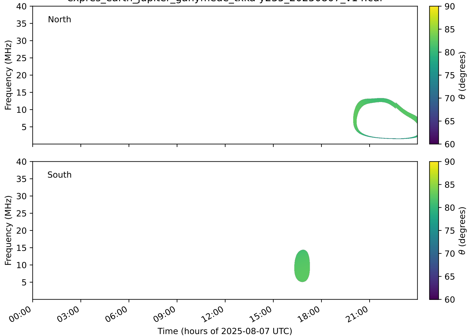
expres_earth_jupiter_ganymede_txka-y235_20250807_v14.cdf
