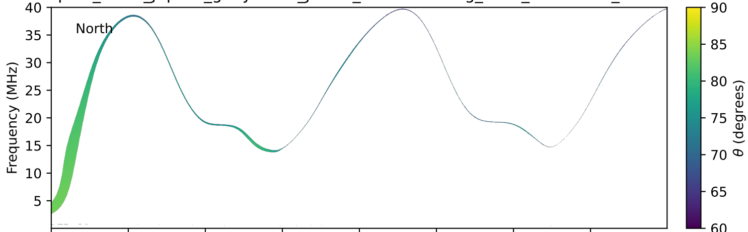
expres_earth_jupiter_ganymede_jrm33_lossc-wid1deg_3kev_20250830_v11.cdf
