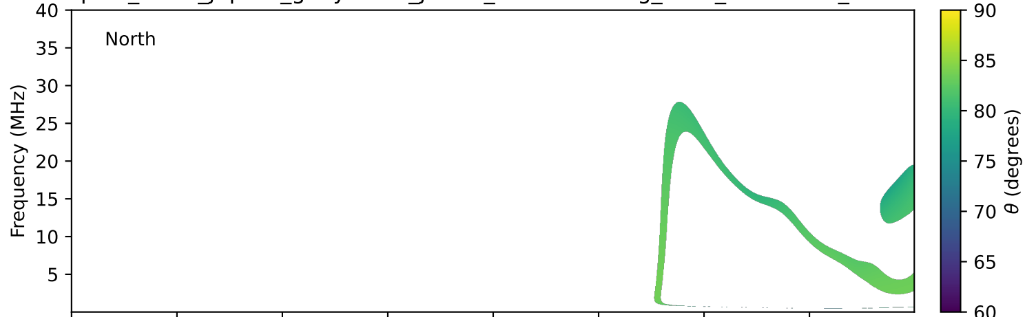
expres_earth_jupiter_ganymede_jrm33_lossc-wid1deg_3kev_20250829_v11.cdf
