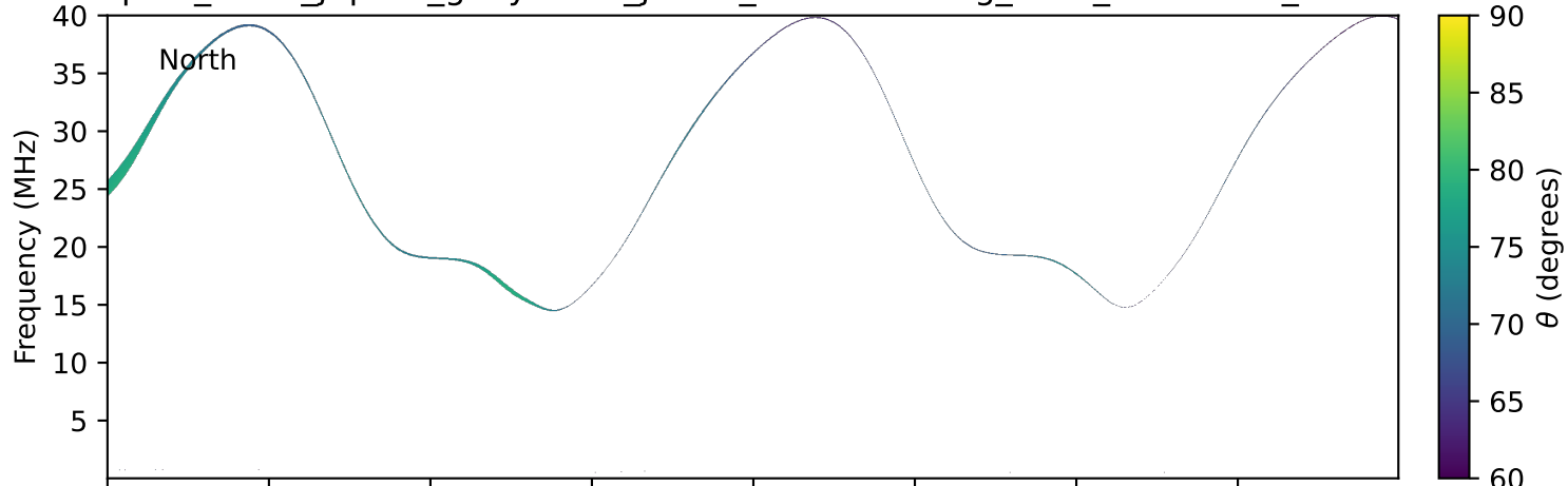
expres_earth_jupiter_ganymede_jrm33_lossc-wid1deg_3kev_20250823_v11.cdf
