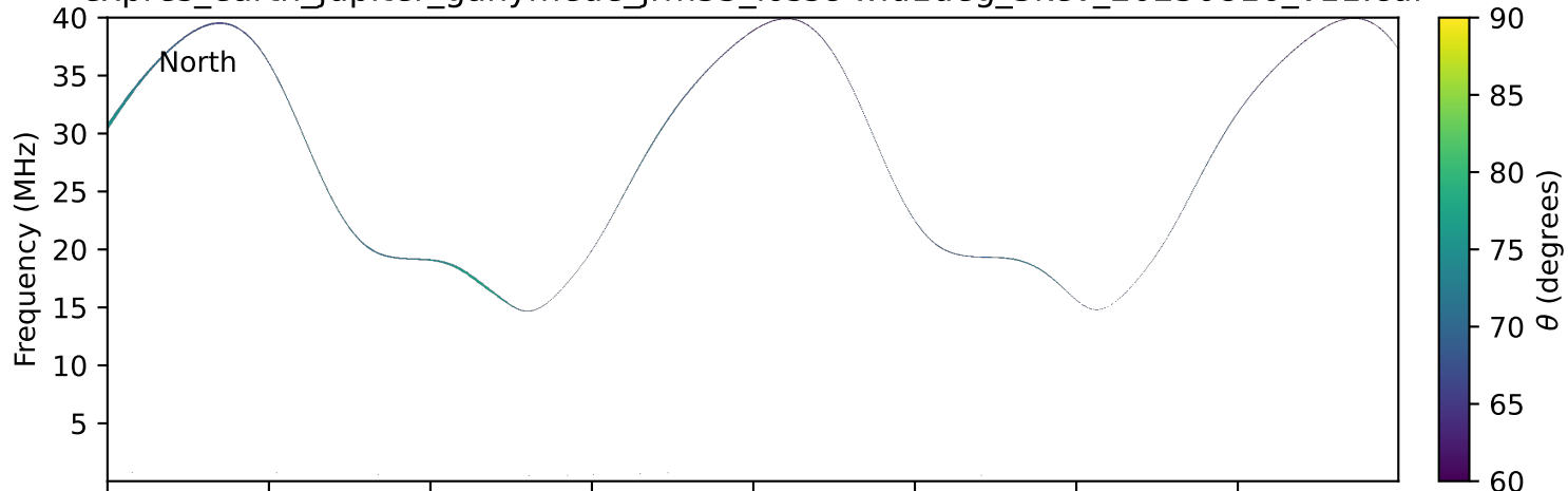
expres_earth_jupiter_ganymede_jrm33_lossc-wid1deg_3kev_20250816_v11.cdf
