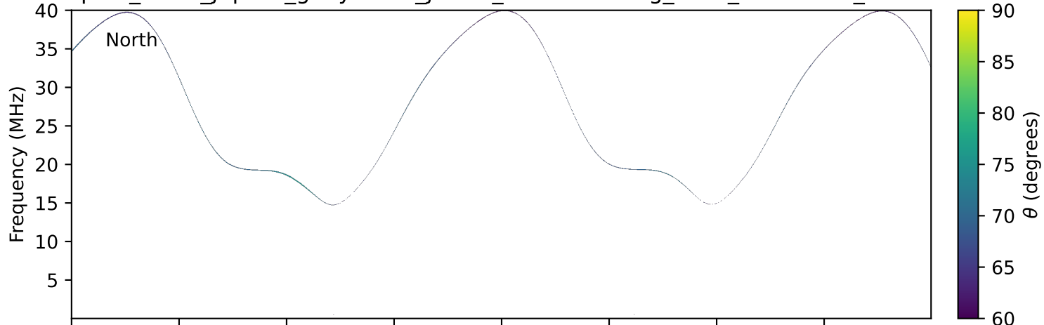
expres_earth_jupiter_ganymede_jrm33_lossc-wid1deg_3kev_20250809_v11.cdf
