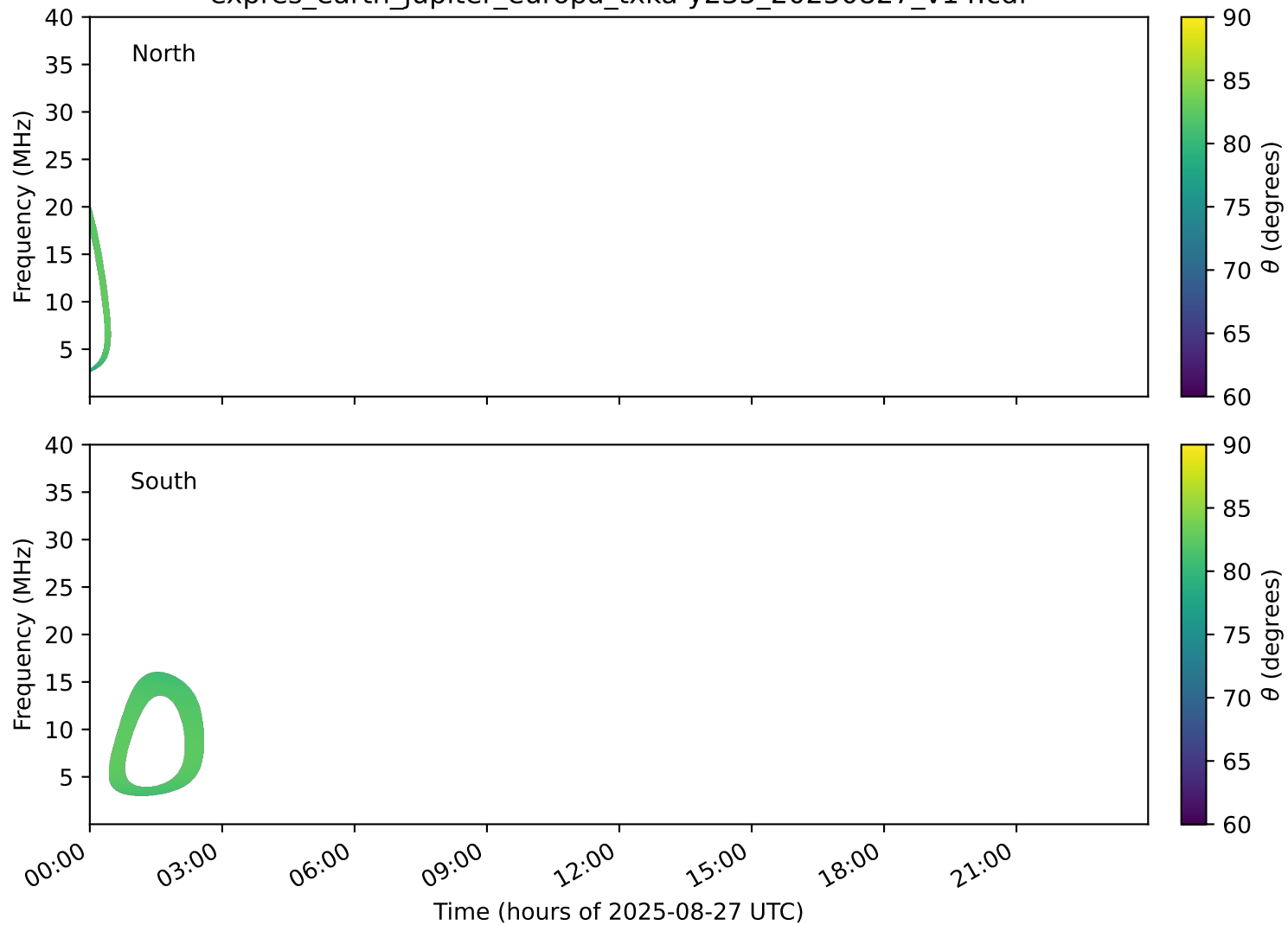
expres_earth_jupiter_europa_txka-y235_20250827_v14.cdf
