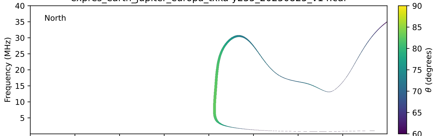
expres_earth_jupiter_europa_txka-y235_20250825_v14.cdf
