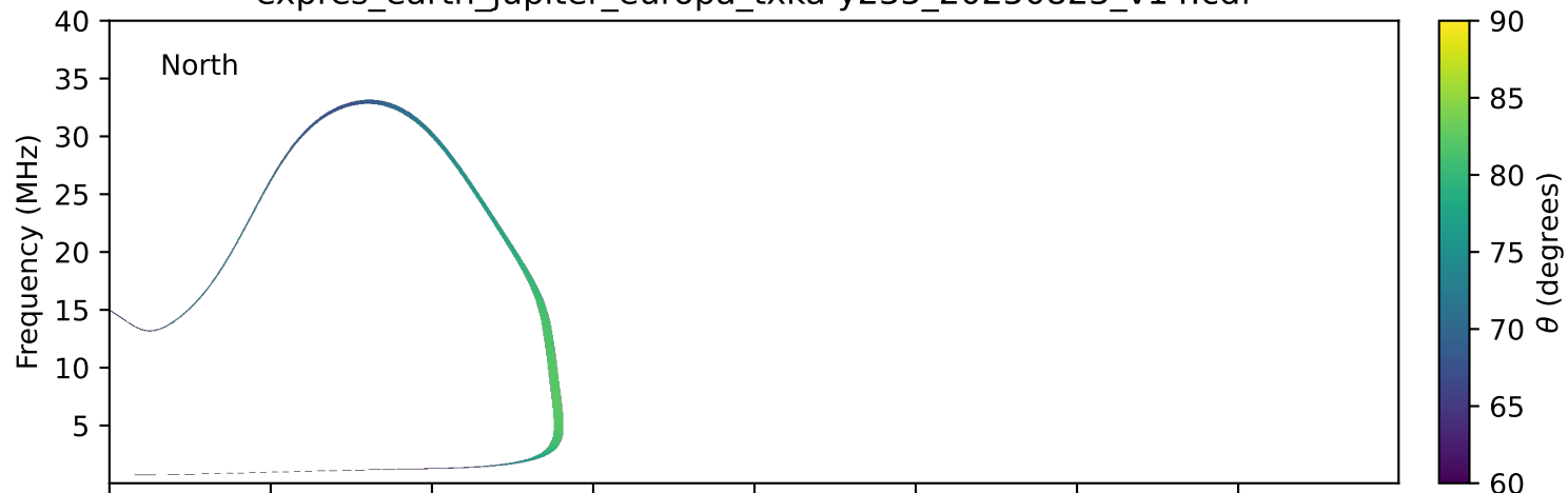
expres_earth_jupiter_europa_txka-y235_20250823_v14.cdf
