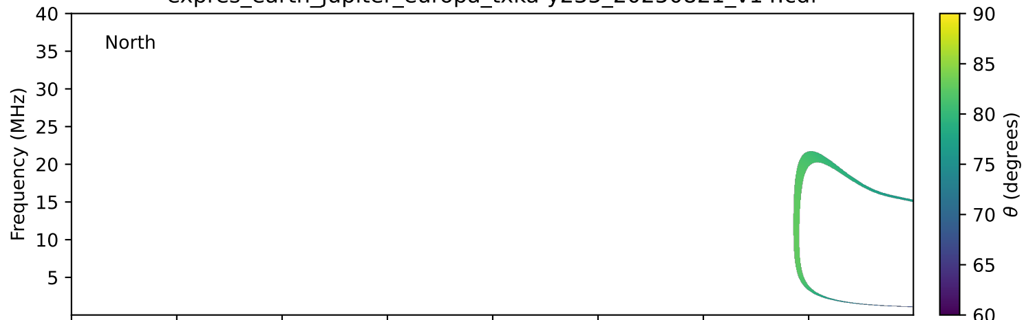
expres_earth_jupiter_europa_txka-y235_20250821_v14.cdf
