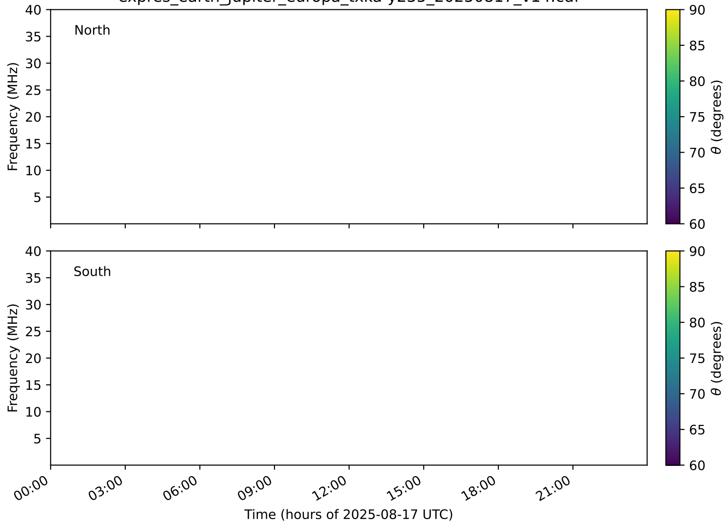
expres_earth_jupiter_europa_txka-y235_20250817_v14.cdf
