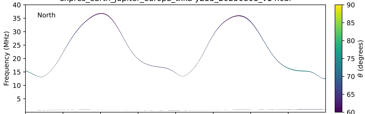
expres_earth_jupiter_europa_txka-y235_20250808_v14.cdf
