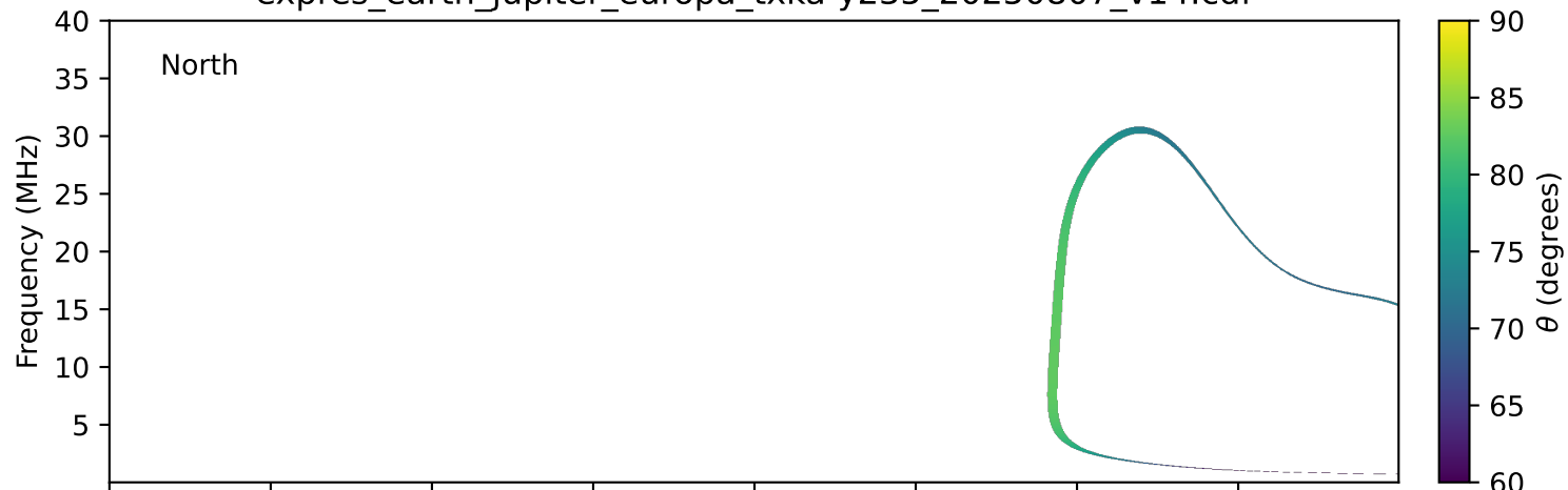
expres_earth_jupiter_europa_txka-y235_20250807_v14.cdf
