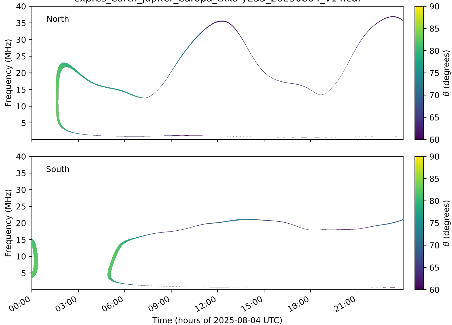
expres_earth_jupiter_europa_txka-y235_20250804_v14.cdf
