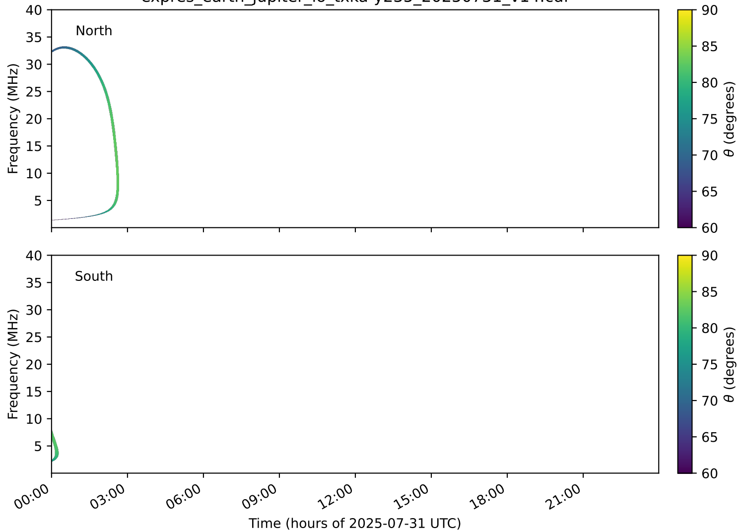
expres_earth_jupiter_io_txka-y235_20250731_v14.cdf
