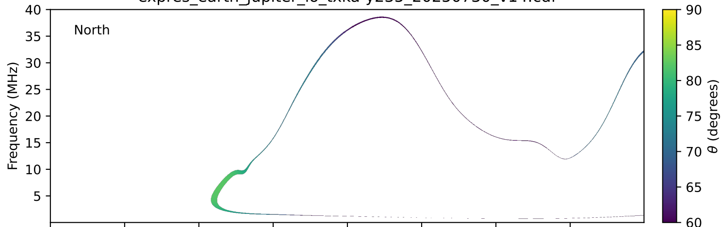
expres_earth_jupiter_io_txka-y235_20250730_v14.cdf
