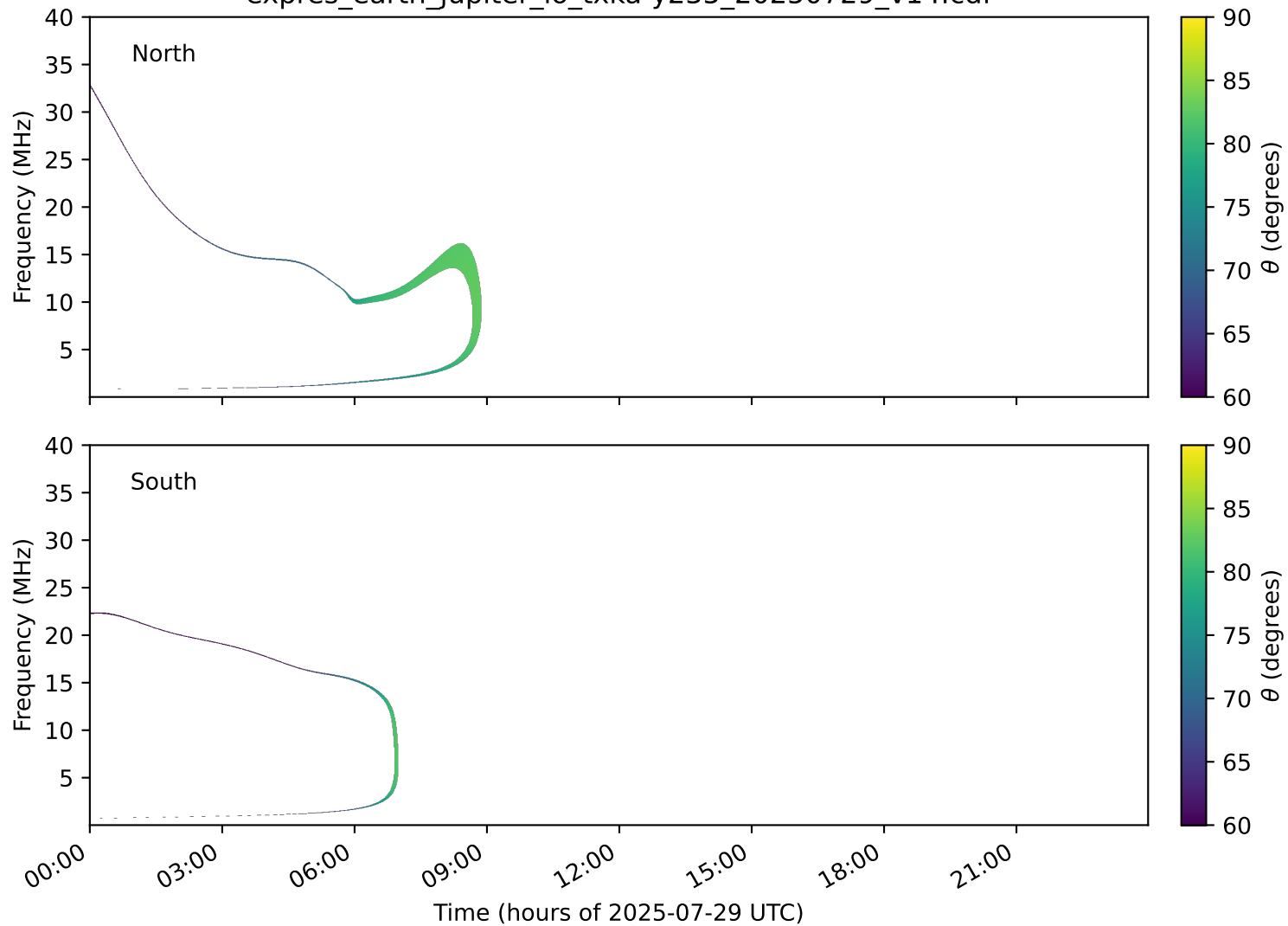
expres_earth_jupiter_io_txka-y235_20250729_v14.cdf
