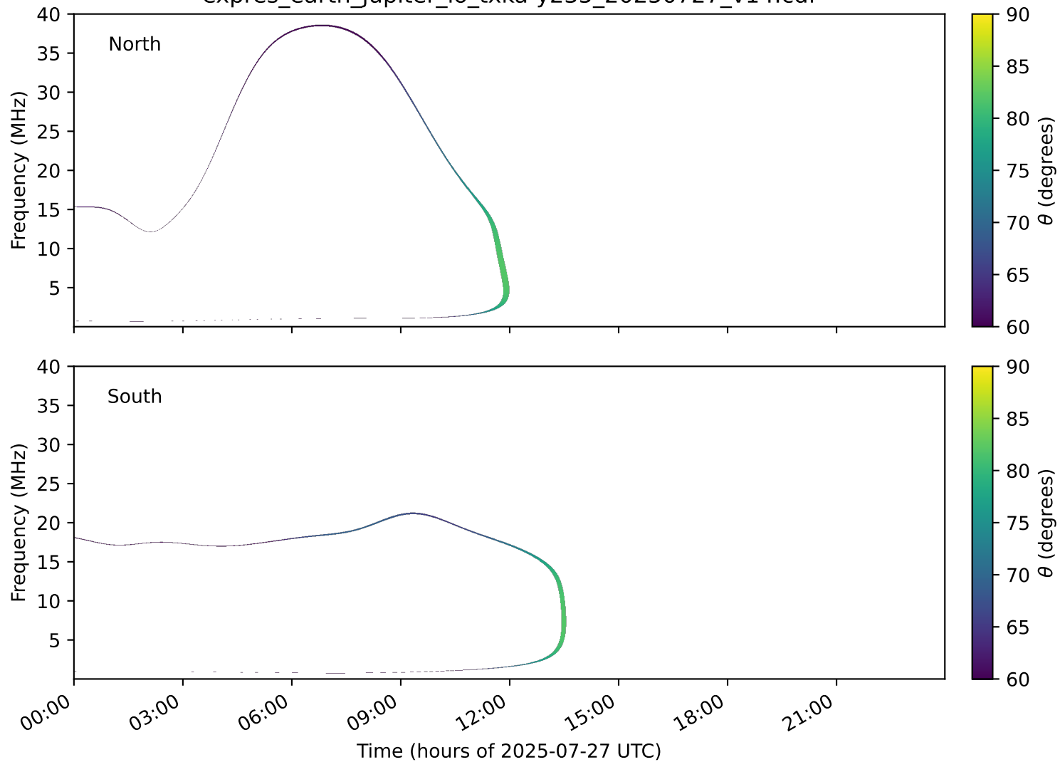
expres_earth_jupiter_io_txka-y235_20250727_v14.cdf
