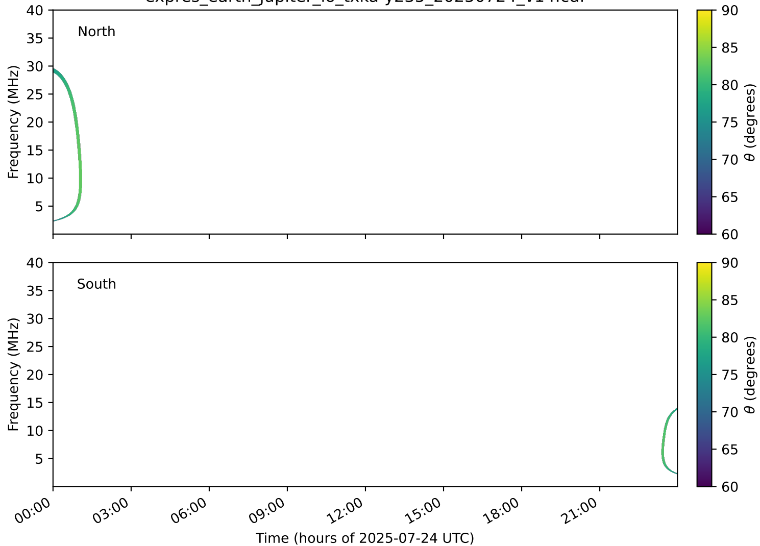
expres_earth_jupiter_io_txka-y235_20250724_v14.cdf
