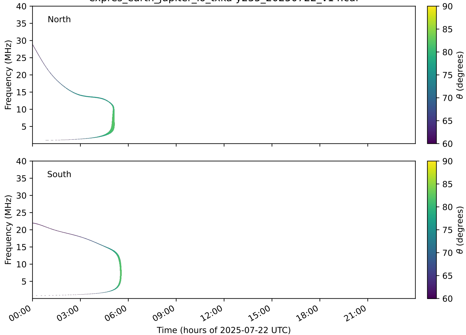
expres_earth_jupiter_io_txka-y235_20250722_v14.cdf
