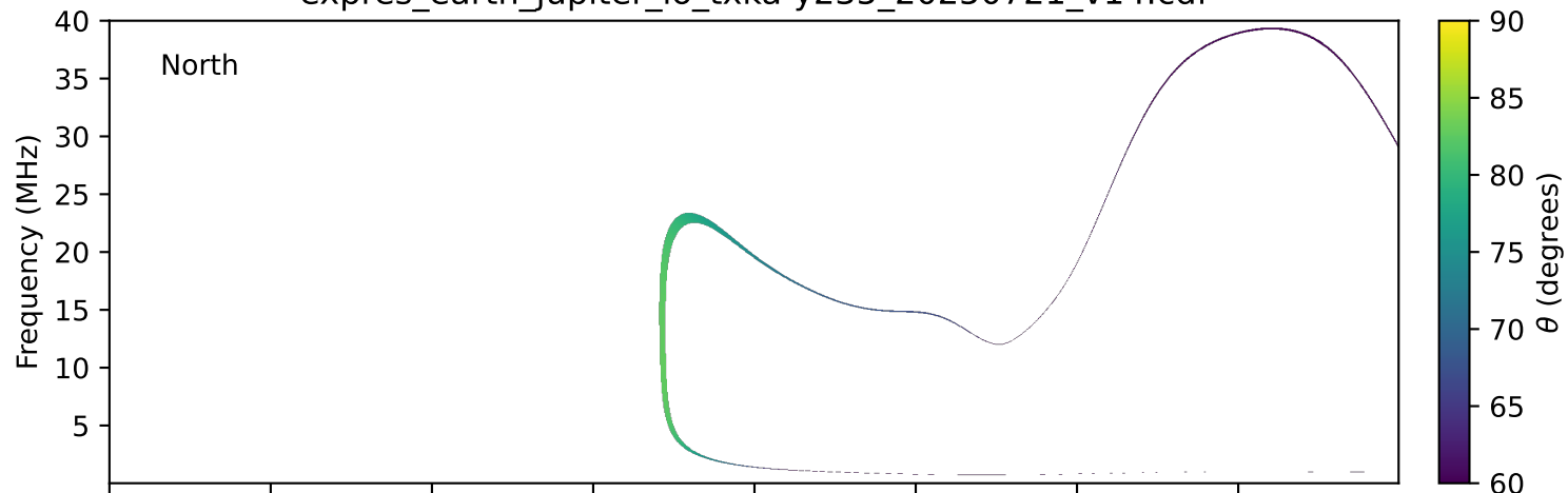
expres_earth_jupiter_io_txka-y235_20250721_v14.cdf
