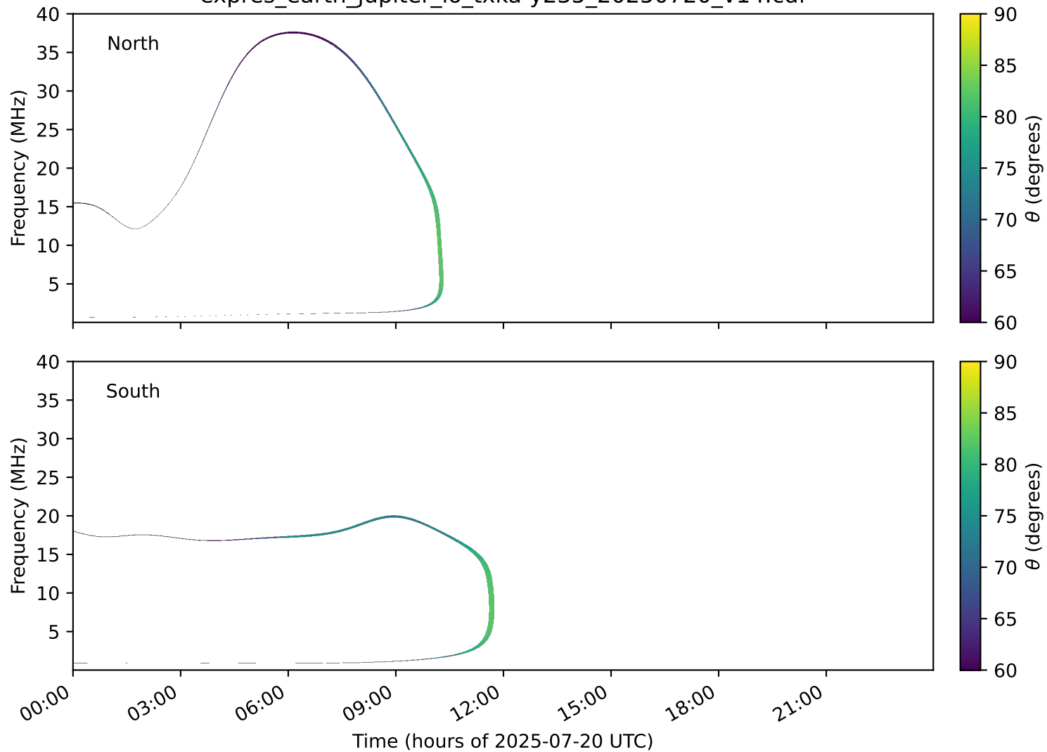
expres_earth_jupiter_io_txka-y235_20250720_v14.cdf
