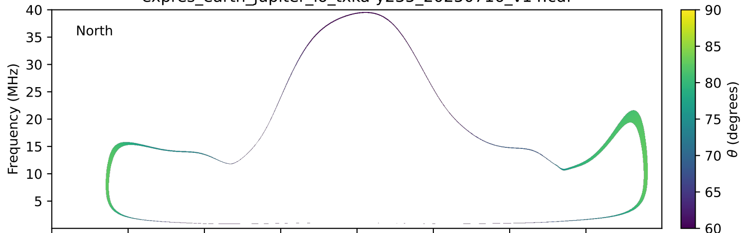
expres_earth_jupiter_io_txka-y235_20250716_v14.cdf
