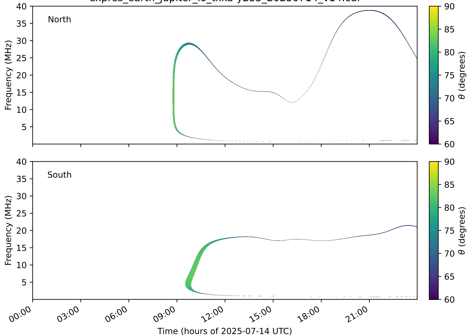
expres_earth_jupiter_io_txka-y235_20250714_v14.cdf
