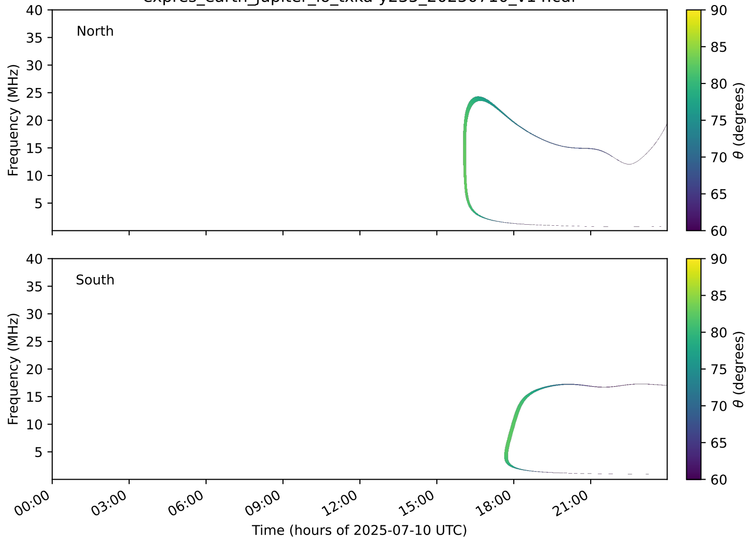
expres_earth_jupiter_io_txka-y235_20250710_v14.cdf
