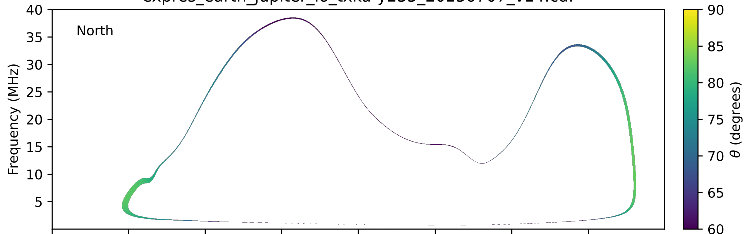
expres_earth_jupiter_io_txka-y235_20250707_v14.cdf
