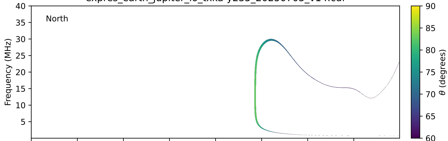
expres_earth_jupiter_io_txka-y235_20250703_v14.cdf
