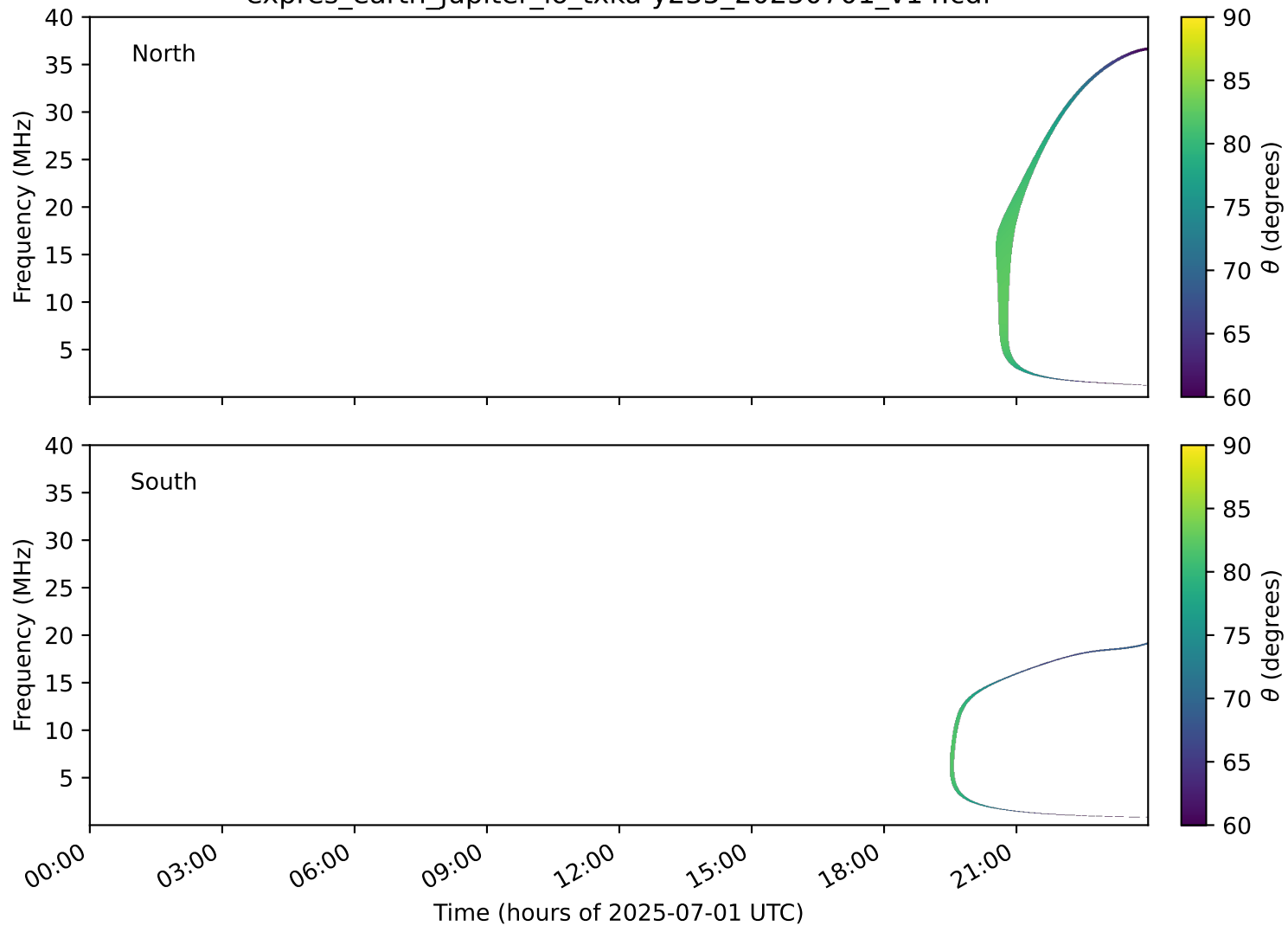
expres_earth_jupiter_io_txka-y235_20250701_v14.cdf
