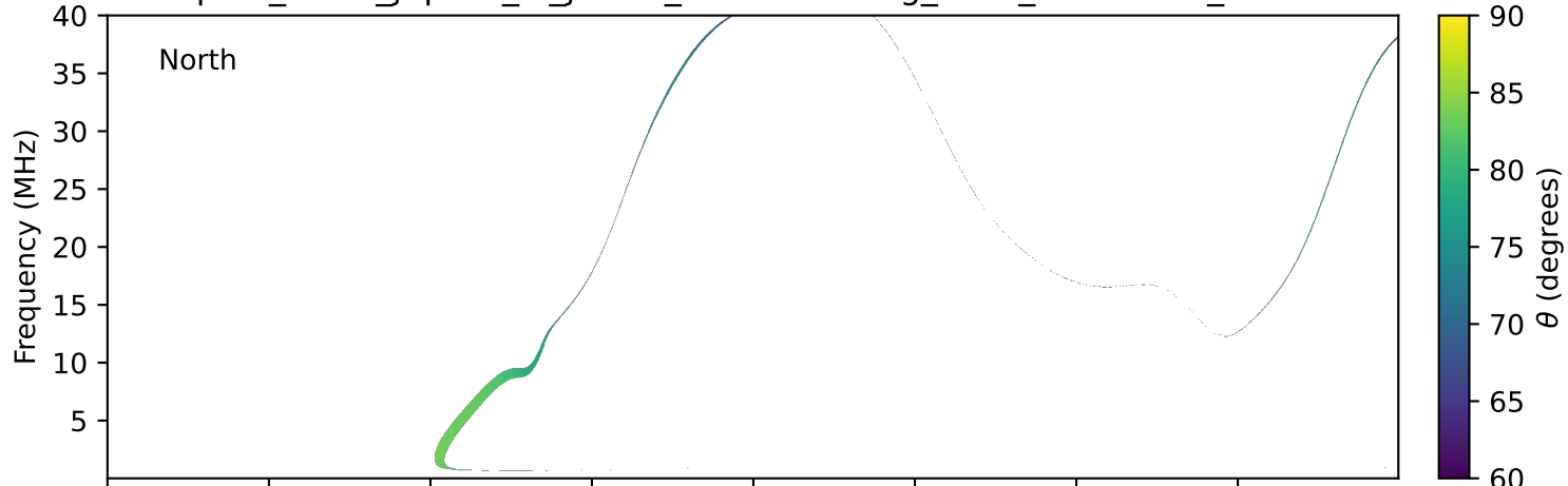
expres_earth_jupiter_io_jrm33_lossc-wid1deg_3kev_20250730_v11.cdf
