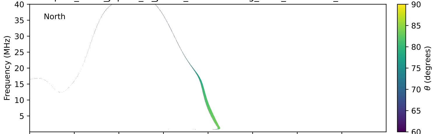
expres_earth_jupiter_io_jrm33_lossc-wid1deg_3kev_20250727_v11.cdf
