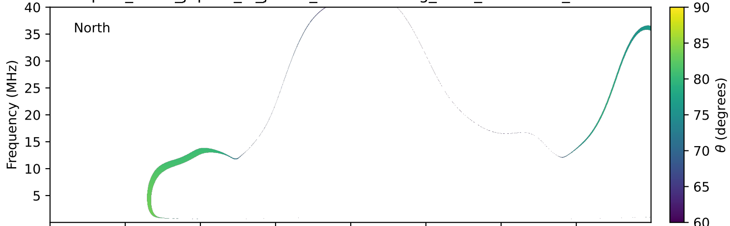
expres_earth_jupiter_io_jrm33_lossc-wid1deg_3kev_20250723_v11.cdf
