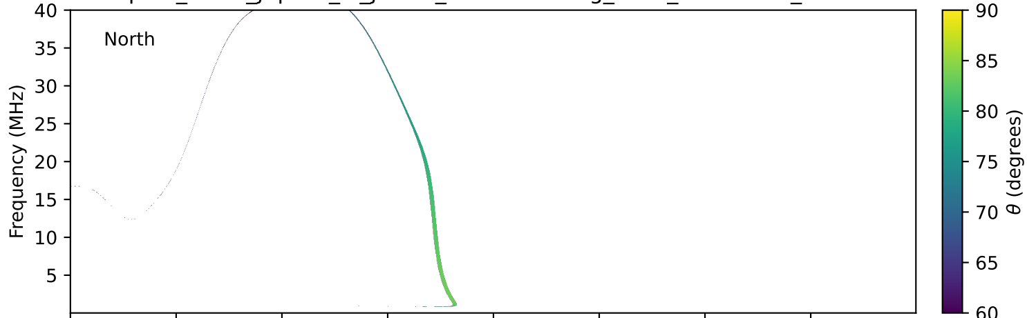
expres_earth_jupiter_io_jrm33_lossc-wid1deg_3kev_20250720_v11.cdf
